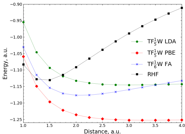
FIG. 3. H_2 SCF potential energy surface for Fermi-Amaldi, LDA, and PBE exchange functionals combined with TF_{\frac{1}{6}}W and TF_{\frac{1}{5}}W kinetic energy functionals, respectively. Calculations were performed with the basis set containing 13 s - and 4 p -functions (see Sec. III D). Self-consistent calculations were performed only at the marked points. The connecting curves are interpolations.
