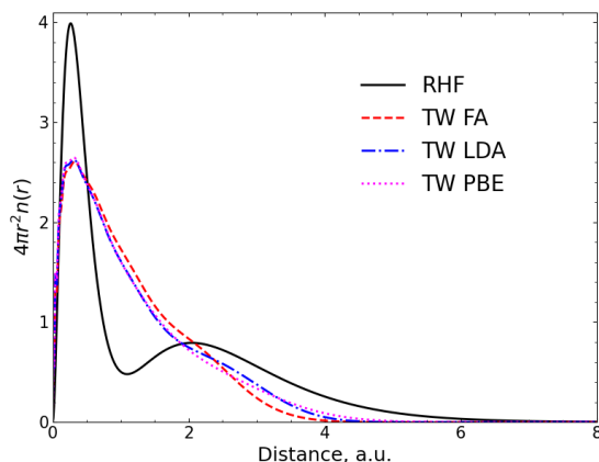
FIG. 4. Be SCF radial distribution function 4\pi r^2 n(\mathbf{r}) for FA, LDA, and PBE exchange functionals combined with TW kinetic energy functional.
