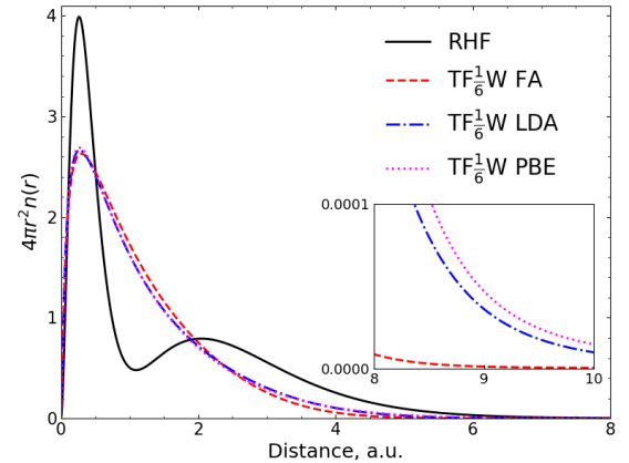
FIG. 2. Be SCF radial distribution function 4\pi r^2 n(\mathbf{r}) for FA, LDA, and PBE exchange functionals combined with \text{TF}_{\frac{1}{6}}\text{W} kinetic energy functional. The RHF reference is included for comparison.
