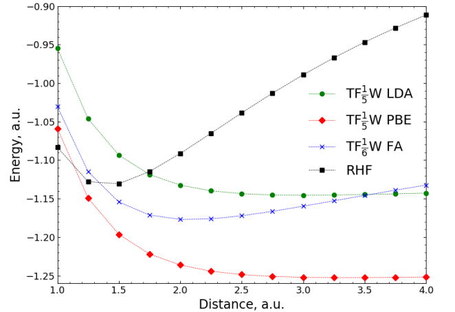
FIG. 5. \text{H}_2 SCF potential energy surface for Fermi-Amaldi, LDA, and PBE exchange functionals combined with \text{TF}_6^{1/2}\text{W} and \text{TF}_5^{1/2}\text{W} kinetic energy functionals, respectively. Calculations were performed with the basis set containing 13 s - and 4 p -functions (see Sec. III D). Self-consistent calculations were performed only at the marked points. The connecting curves are interpolations.
