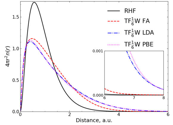
FIG. 1. He SCF radial distribution function 4\pi r^2 n(\mathbf{r}) for FA, LDA, and PBE exchange functionals combined with \text{TF}_{\frac{1}{6}}\text{W} kinetic energy functional. The RHF reference is included for comparison.
