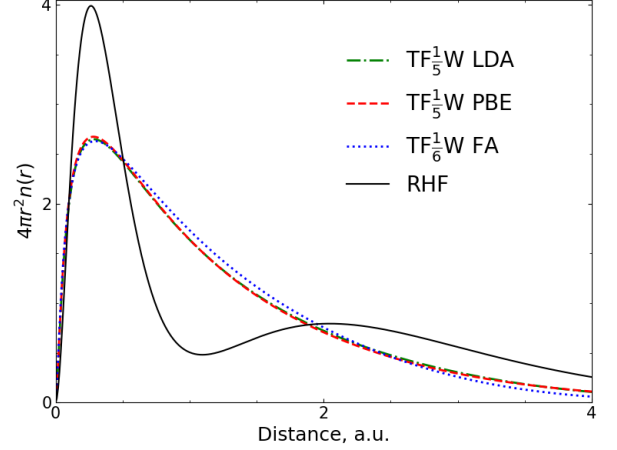
FIG. 1. Be SCF radial distribution function 4\pi r^2 n(\mathbf{r}) for Fermi-Amaldi, LDA, and PBE exchange functionals combined with \text{TF}_{\frac{1}{6}}\text{W} and \text{TF}_{\frac{1}{5}}\text{W} kinetic energy functionals, respectively. The basis set with 31 s -type basis functions was used. The RHF reference is included for comparison.
