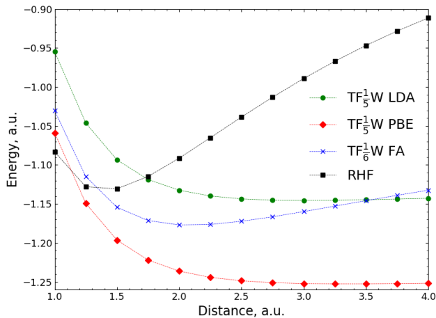
FIG. 2. H_2 SCF potential energy surface for Fermi–Amaldi, LDA, and PBE exchange functionals combined with TF_{\frac{1}{6}}^W and TF_{\frac{1}{5}}^W kinetic energy functionals, respectively. Calculations were performed with the basis set containing 13 s - and 4 p -functions (see Sec. III D). Self-consistent calculations were performed only at the marked points. The connecting curves are interpolations.
