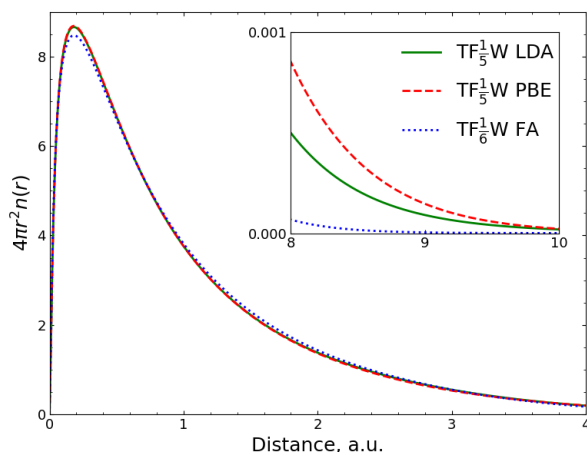
FIG. 1. Ne SCF radial distribution function 4\pi r^2 n(\mathbf{r}) for Fermi–Amaldi, LDA, and PBE exchange functionals combined with \text{TF}_{1/6}\text{W} and \text{TF}_{1/5}\text{W} kinetic energy functionals, respectively. The basis set with 31 s -type basis functions was used (see Sec. III B).
