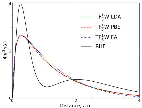
FIG. 1. Be SCF radial distribution function 4\pi r^2 n(r) for Fermi–Amaldi, LDA, and PBE exchange functionals combined with \text{TF}_{\frac{1}{6}}\text{W} and \text{TF}_{\frac{1}{5}}\text{W} kinetic energy functionals, respectively. The basis set with 31 s -type basis functions was used (see Sec. III B). The RHF reference is included for comparison.
