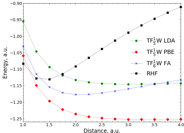
FIG. 2. H_2 SCF potential energy surface for Fermi–Amaldi, LDA, and PBE exchange functionals combined with TF_{\frac{1}{6}}W and TF_{\frac{1}{5}}W kinetic energy functionals, respectively. Calculations were performed with the basis set containing 13 s - and 4 p -functions (see Sec. III D). Self-consistent calculations were performed only at the marked points. The connecting curves are interpolations.
