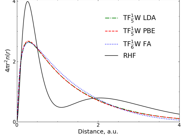
FIG. 1. Be SCF radial distribution function 4\pi r^2 n(\mathbf{r}) for Fermi-Amaldi, LDA, and PBE exchange functionals combined with TF \frac{1}{6} W and TF \frac{1}{5} W kinetic energy functionals, respectively. The basis set with 31 s -type basis functions was used. The RHF reference is included for comparison.
