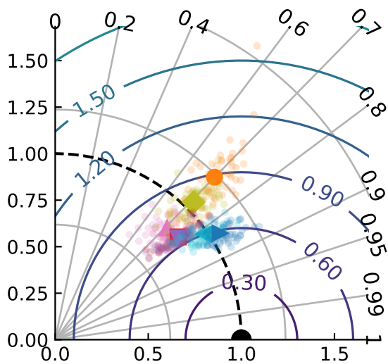
CanESM5
