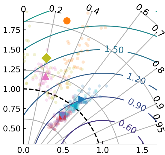
CanESM5
