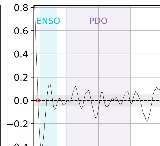
Internal ACF
