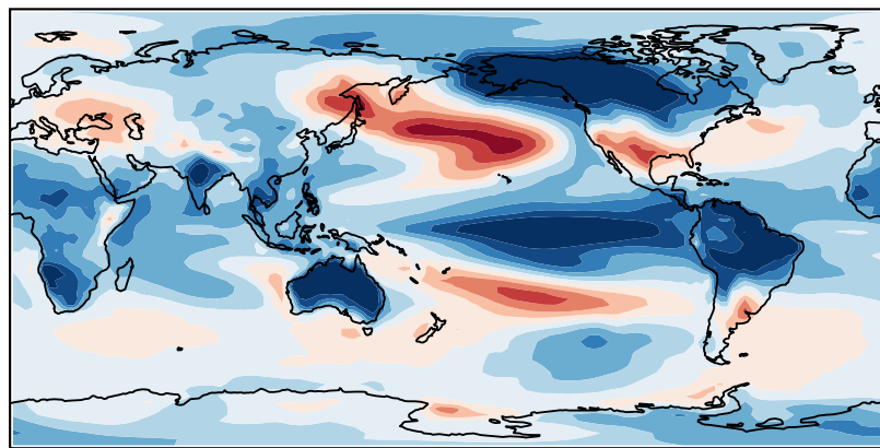
Spatial pattern
