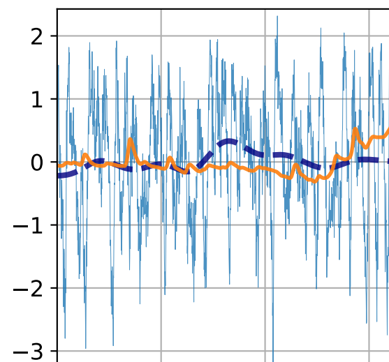
Time series
