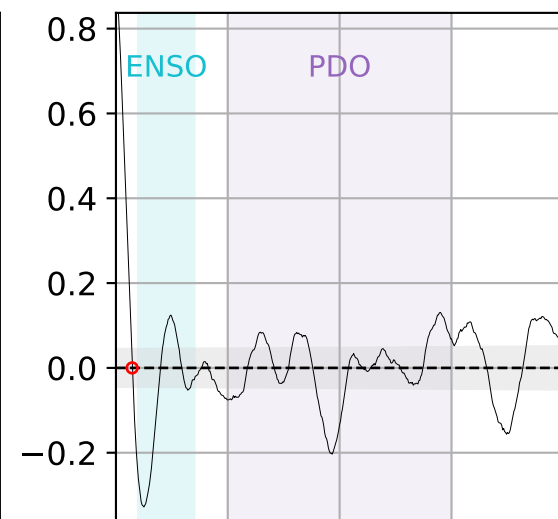
Internal ACF
