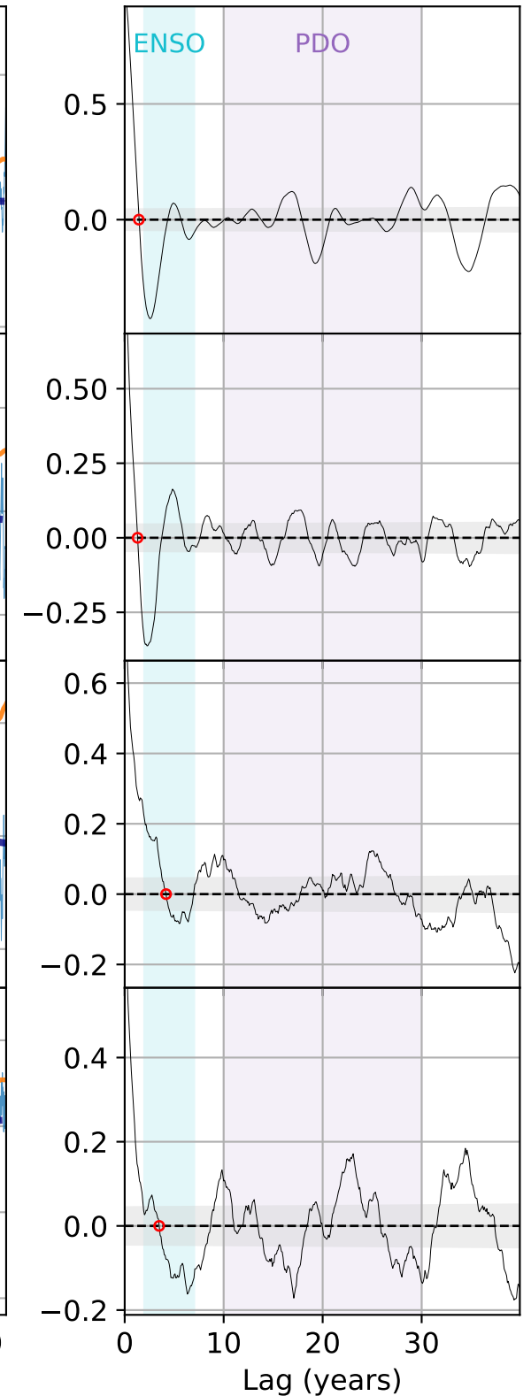
Internal ACF
