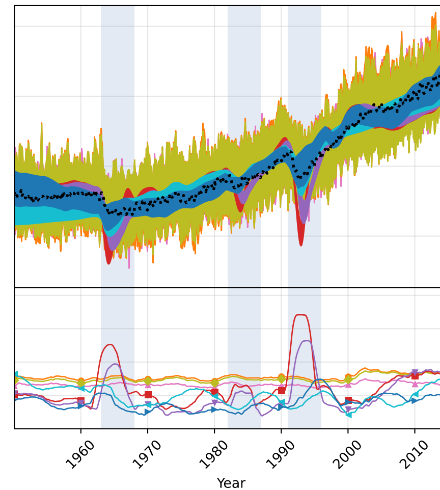
CanESM5
