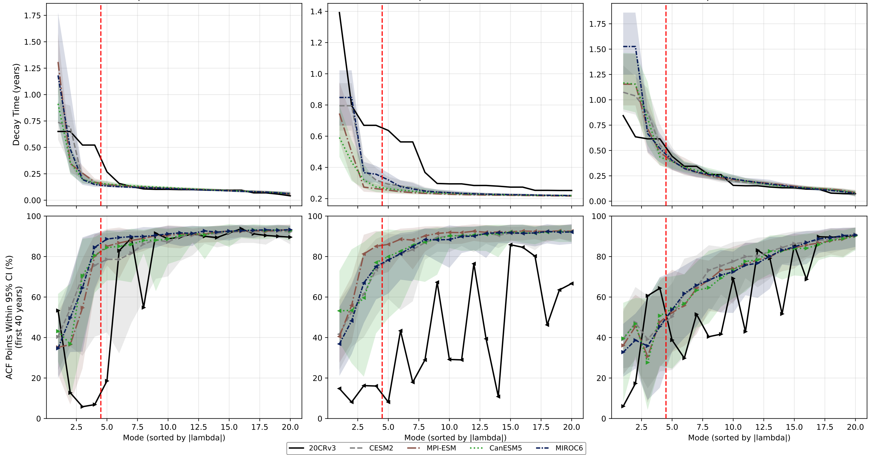
SAT | PullbackDMDc(3d)
