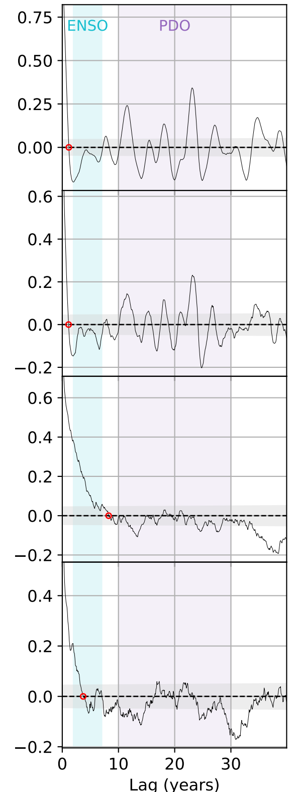
Internal ACF
