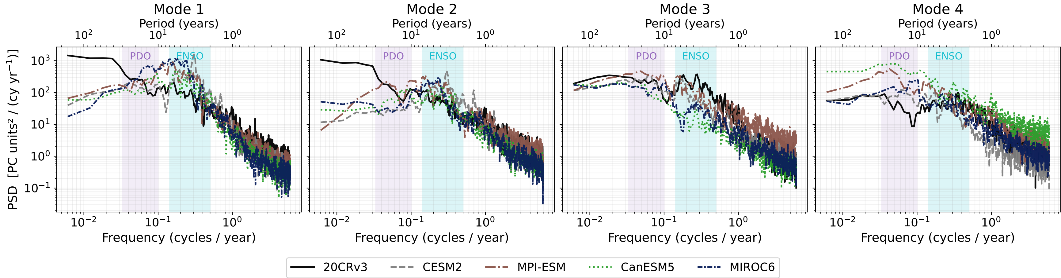
OSAT: Power spectral density - Multitaper MTM, NW=3, K=5 tapers - resolution 0.036 cy/yr (28 yr period)
