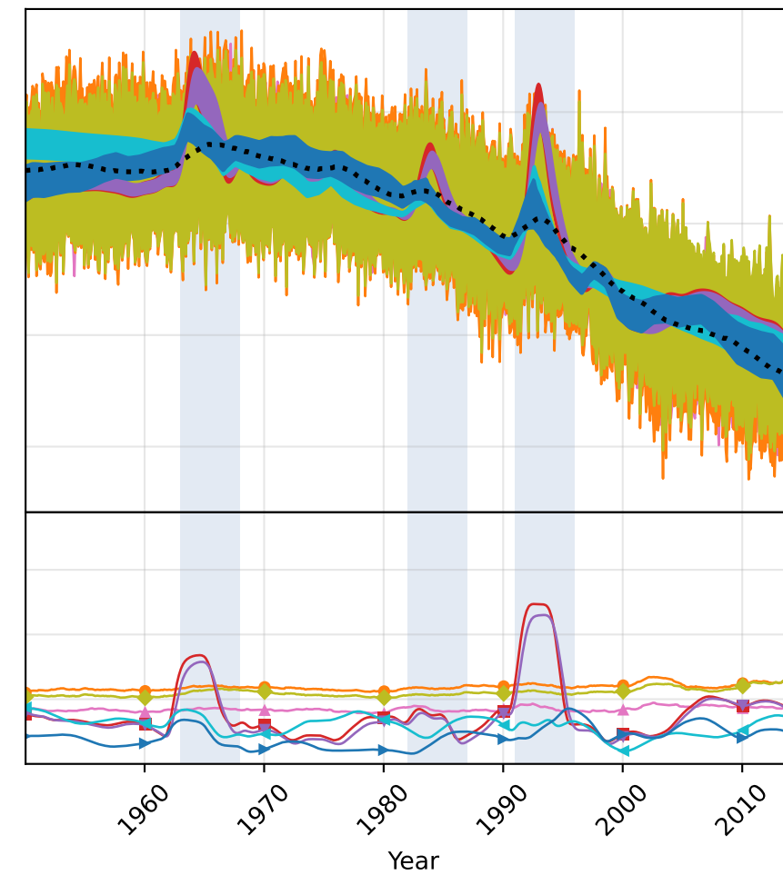
CanESM5
