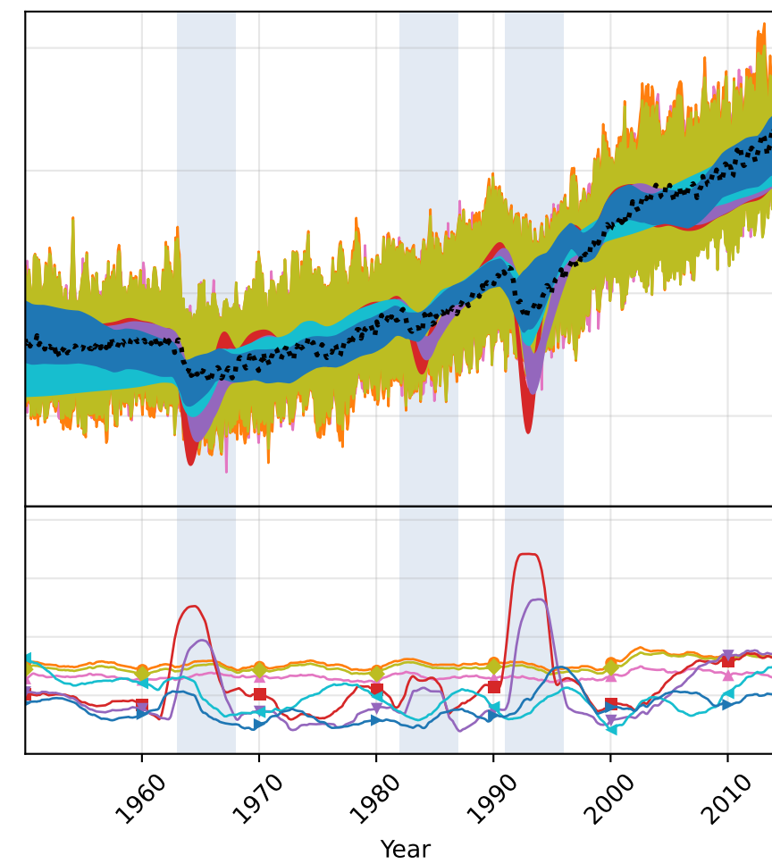
CanESM5
