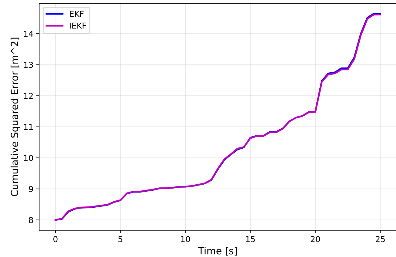
Cumulative Position Error
