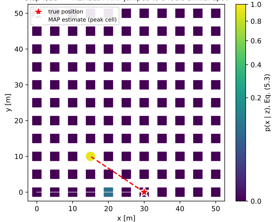
Fingerprint posterior, Section 5.2 (noise 6 dB): the median is 0 m, the mean is not -- aliasing hides in the mean
