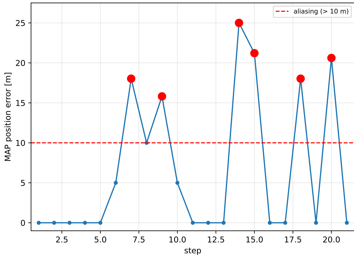
Fingerprint posterior, Section 5.2 (noise 6 dB): the median is 0 m, the mean is not -- aliasing hides in the mean
