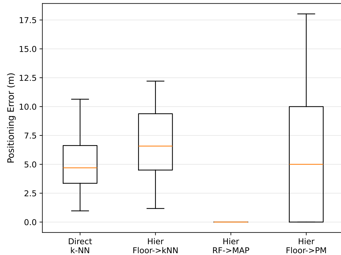
Error Distribution (Box Plot)
