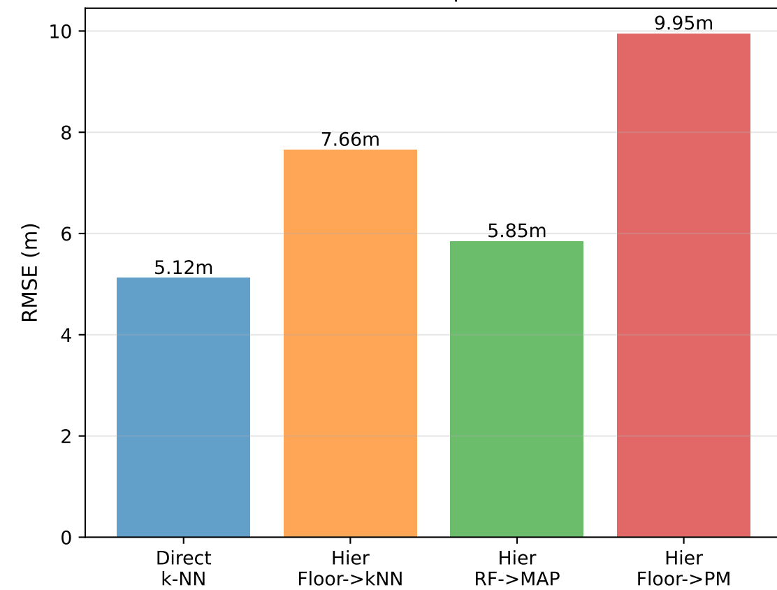
RMSE Comparison
