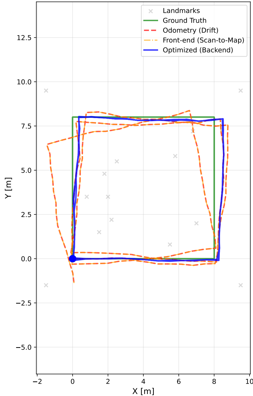
4 Trajectories: Truth / Odom / Front-end / Optimized
