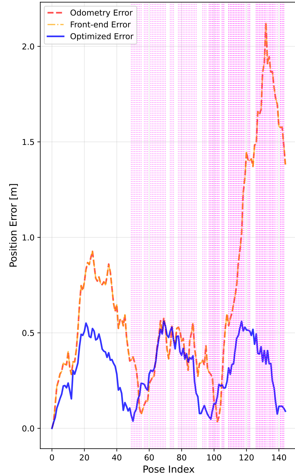
Position Error Over Time
