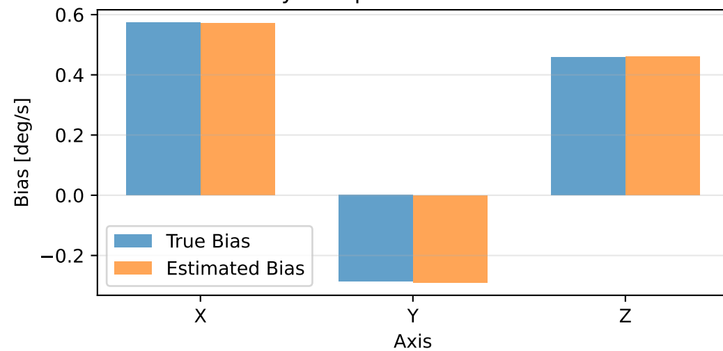
Gyroscope Bias Estimation
