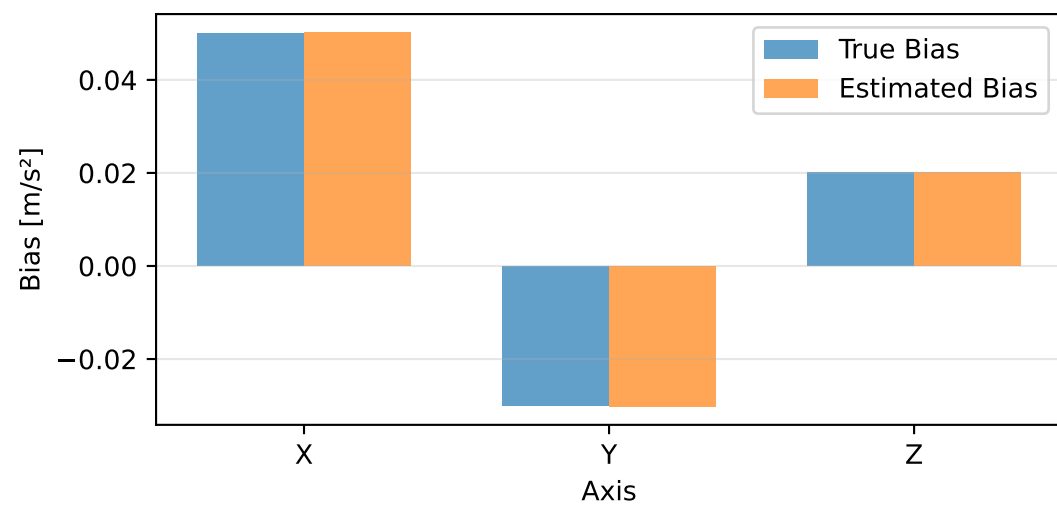
Accelerometer Bias Estimation
