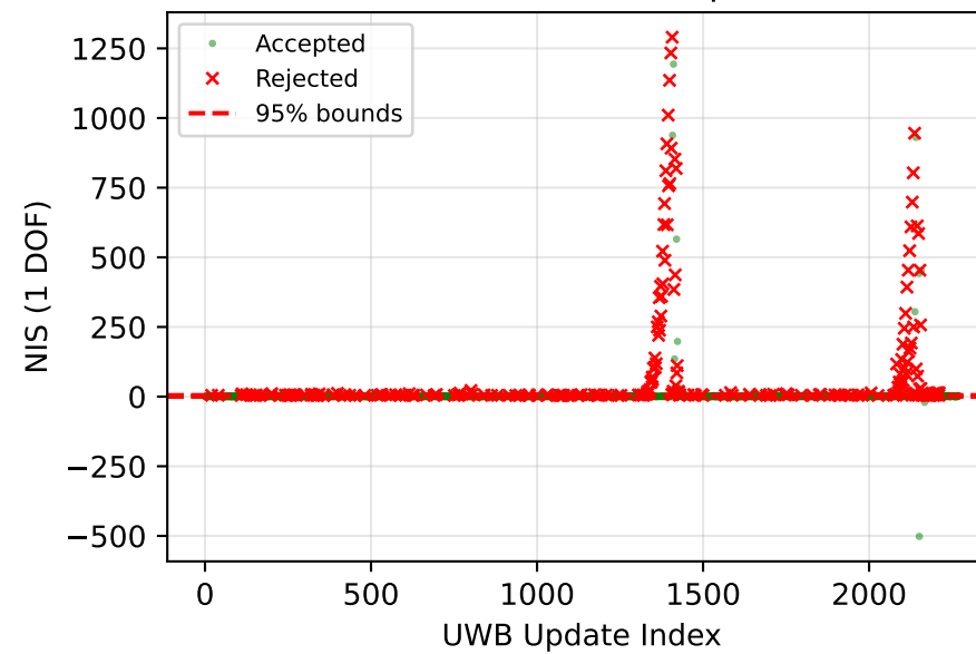
TC NIS (89.4% accepted)
