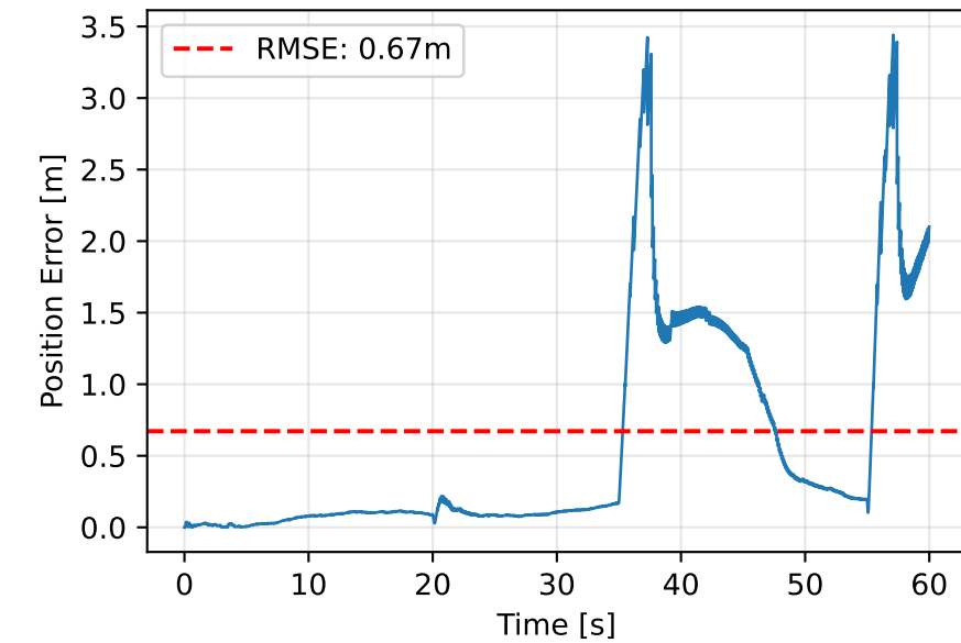
LC NIS (95.9% accepted)
