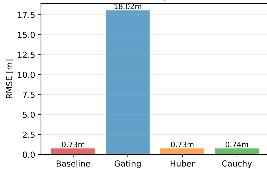
RMSE Comparison
