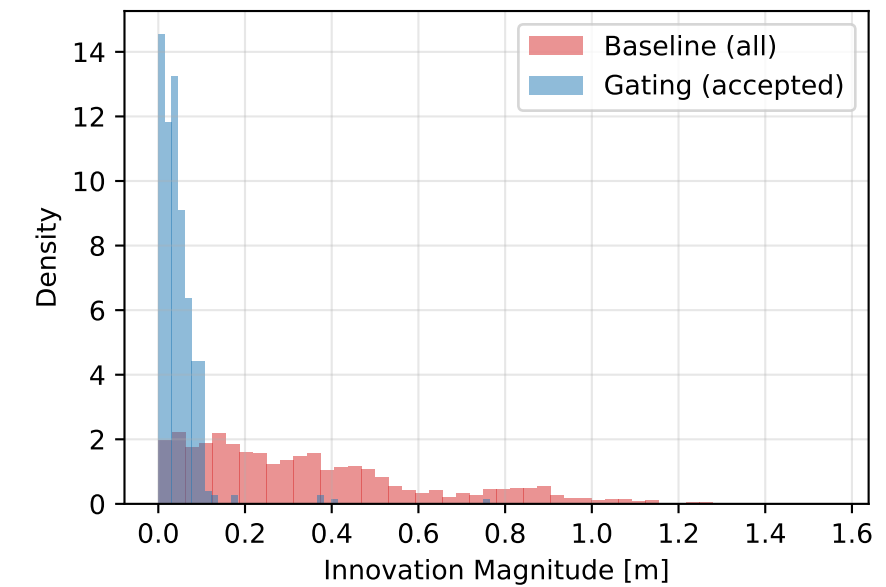
Innovation Distribution
