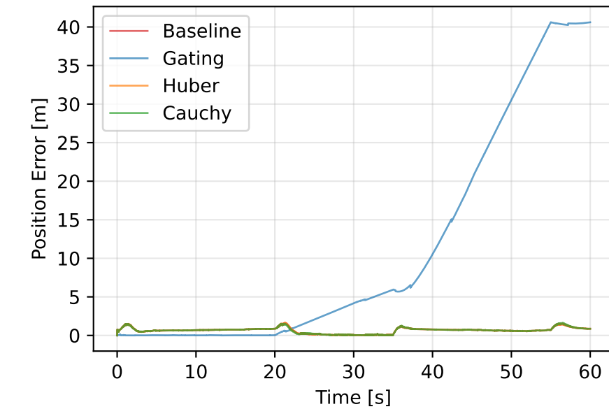
RMSE Comparison
