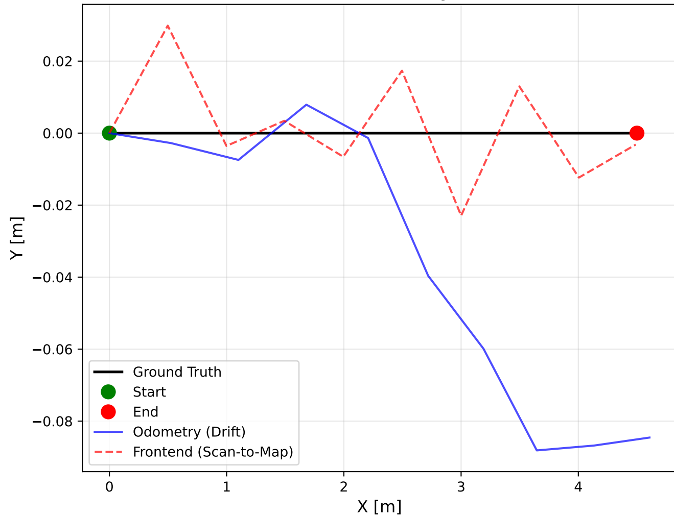
SLAM Front-End: Trajectories
