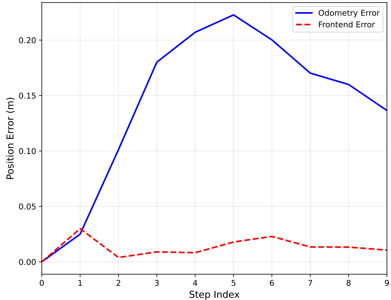
Position Error Over Time
