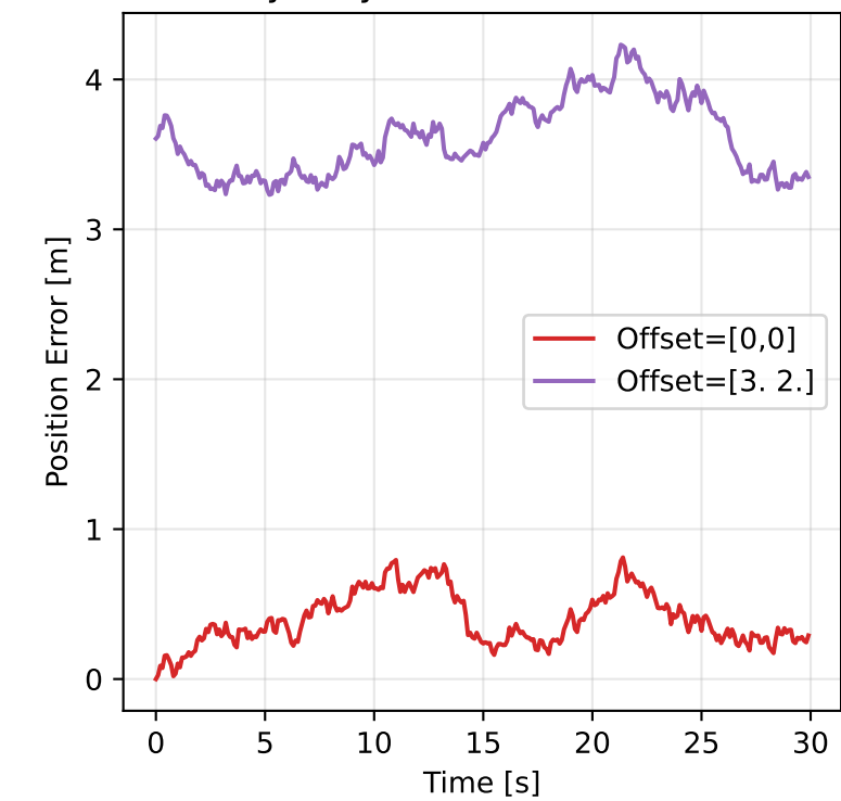
Odometry-Only: Constant Translation Error
