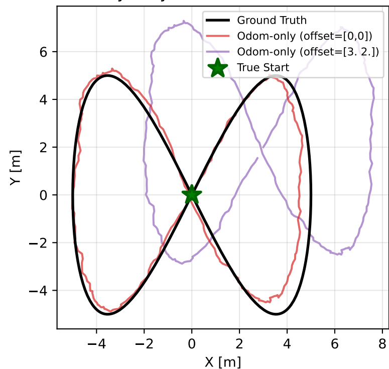
Odometry-Only: Translation is Unobservable
