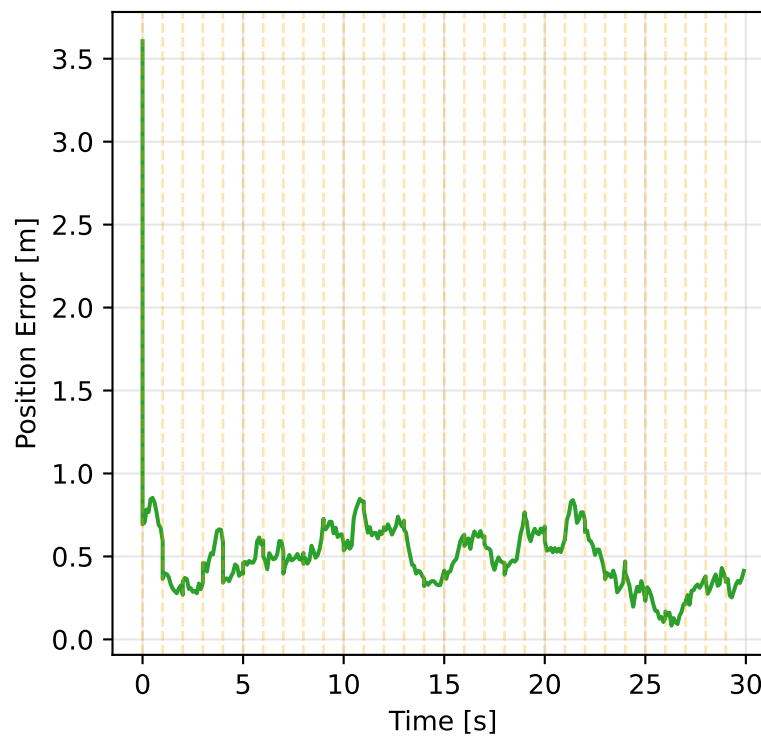
Odom + Fixes: Error Corrected at Fixes
