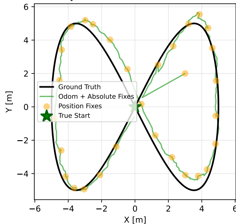
Odometry + Fixes: Translation is Observable
