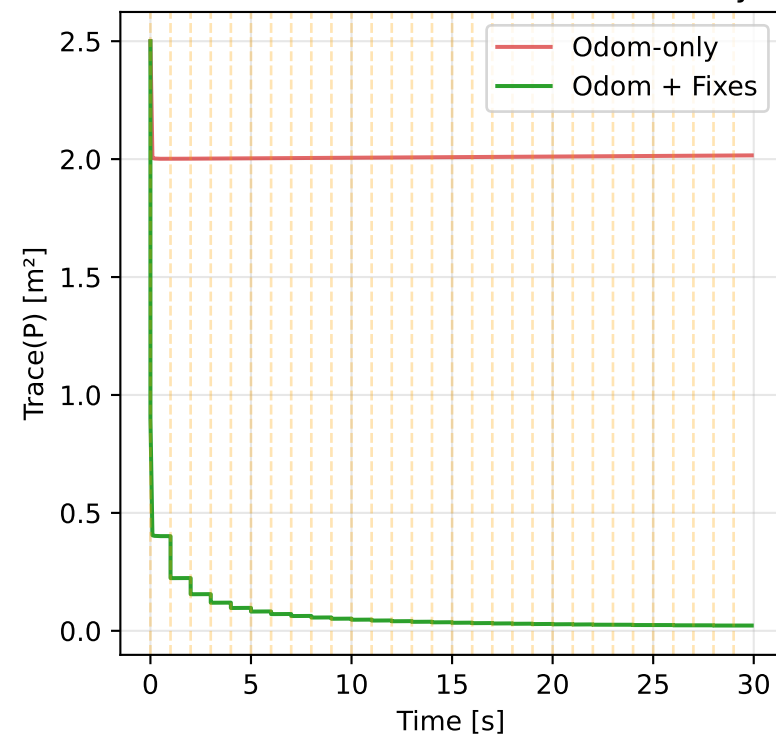
Covariance: Fixes Reduce Uncertainty
