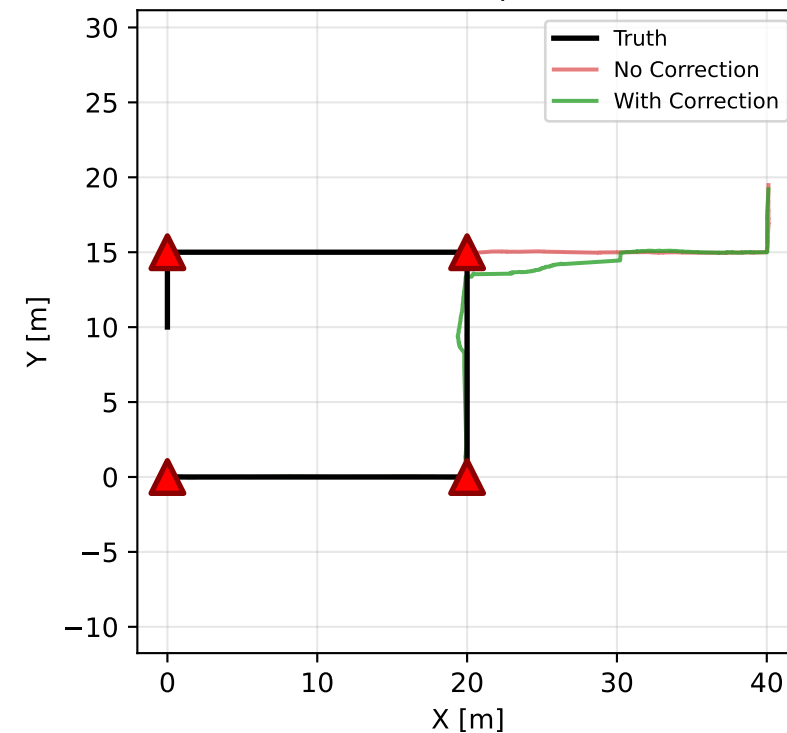
Direct Comparison
