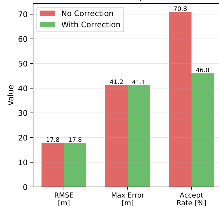
Metrics Comparison
