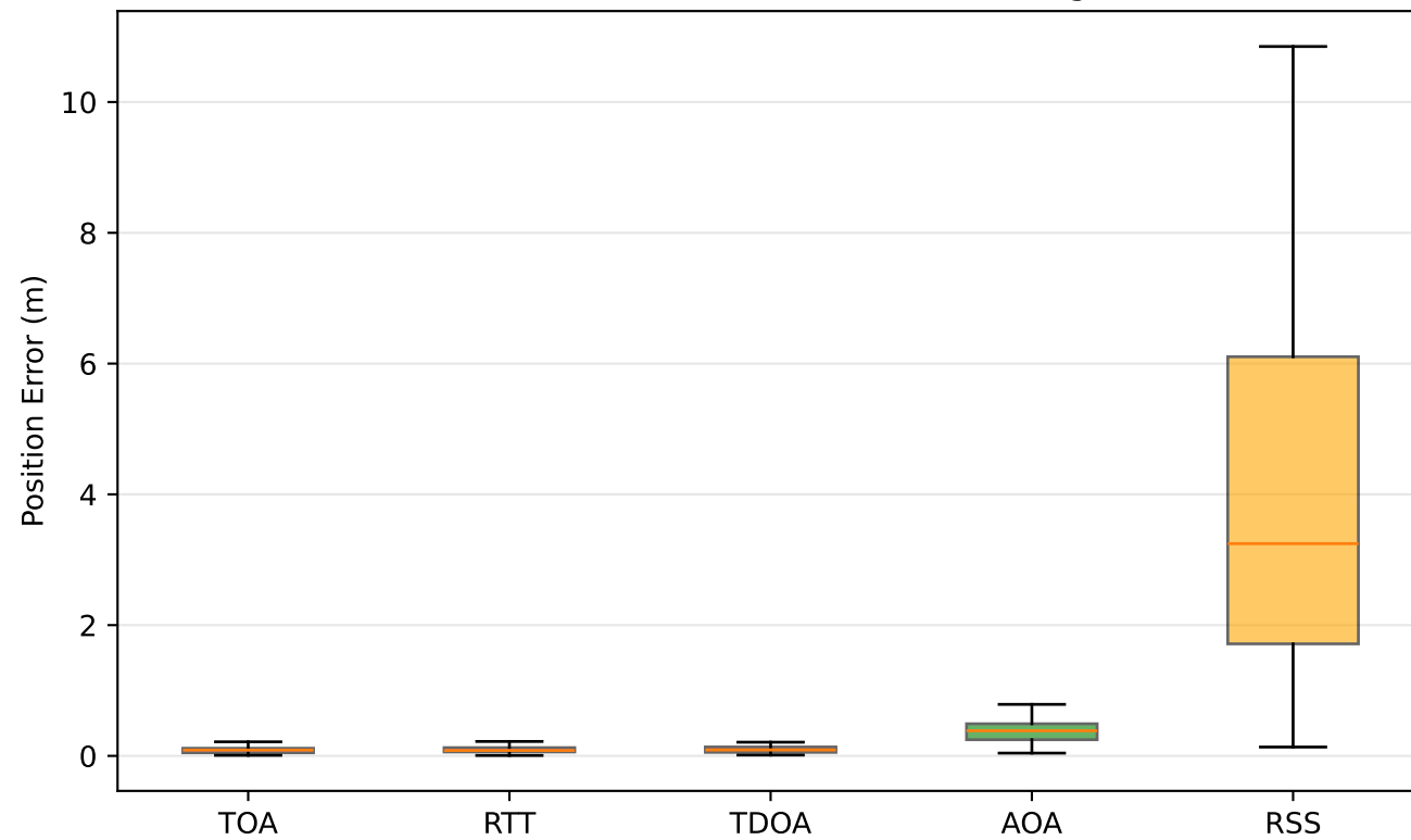
Error distribution at level 3 (TOA 0.1 m, RTT 0.1 m, TDOA 0.1 m, AOA 3 deg, RSS 4 dB)
