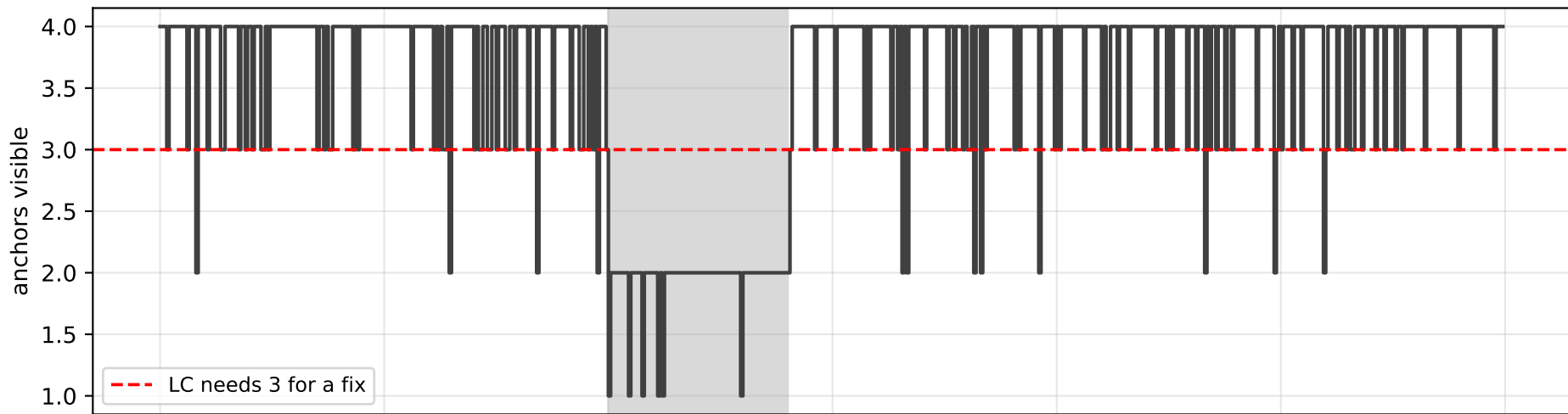
Constructed outage: at most 2 of 4 anchors between t = 20 s and 28 s
