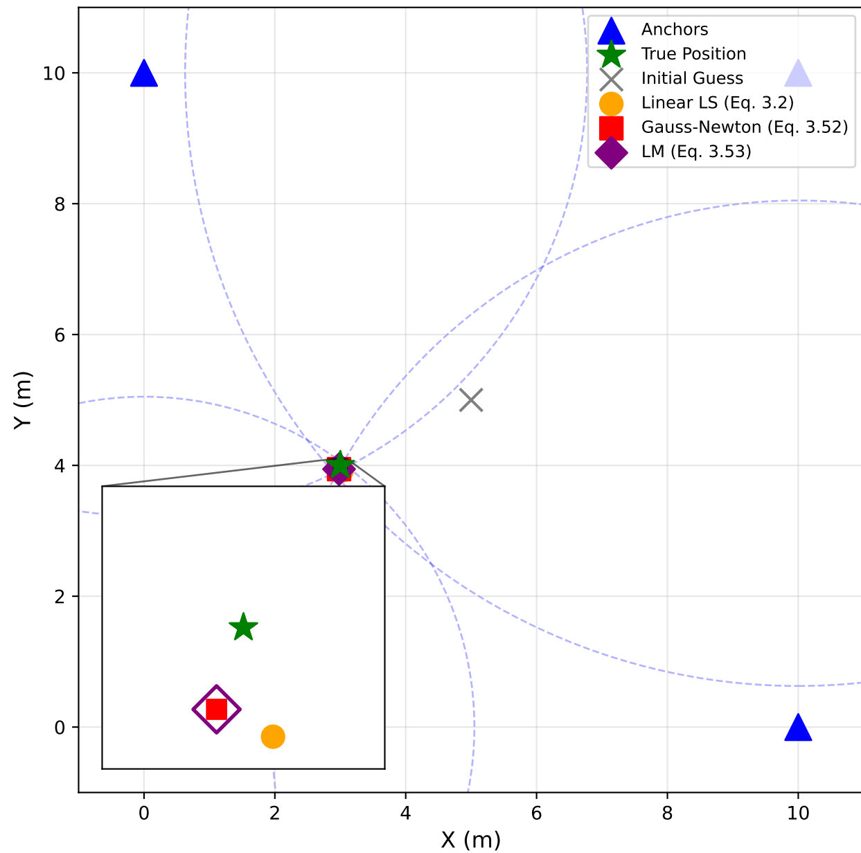
On clean data all three solvers agree to centimetres (inset: a 20 cm window on the same estimates)
