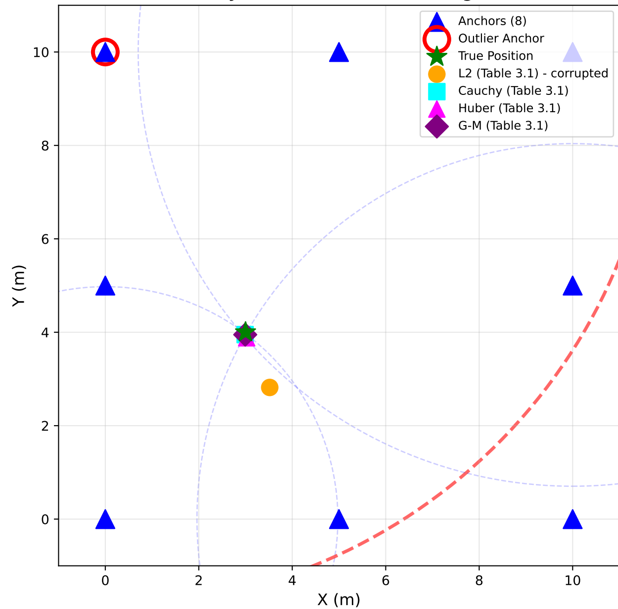
One corrupted anchor drags plain least squares off the truth while every robust loss in Table 3.1 ignores it
