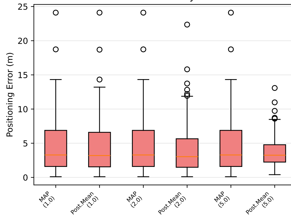
Error Distribution by Method
