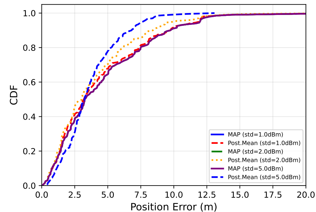
Cumulative Distribution of Errors
