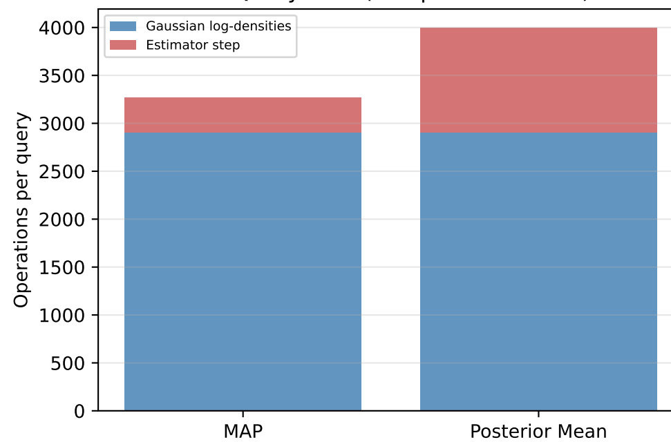
Per-Query Cost (independent of std)
