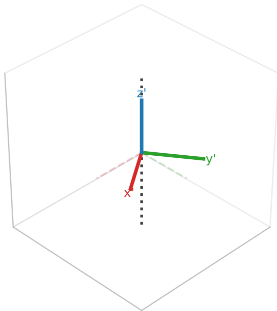
Yaw \psi = 35 deg, about Z Eq. (2.14)
