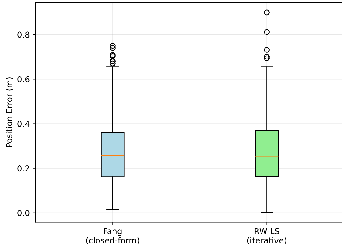
TOA Positioning Comparison
