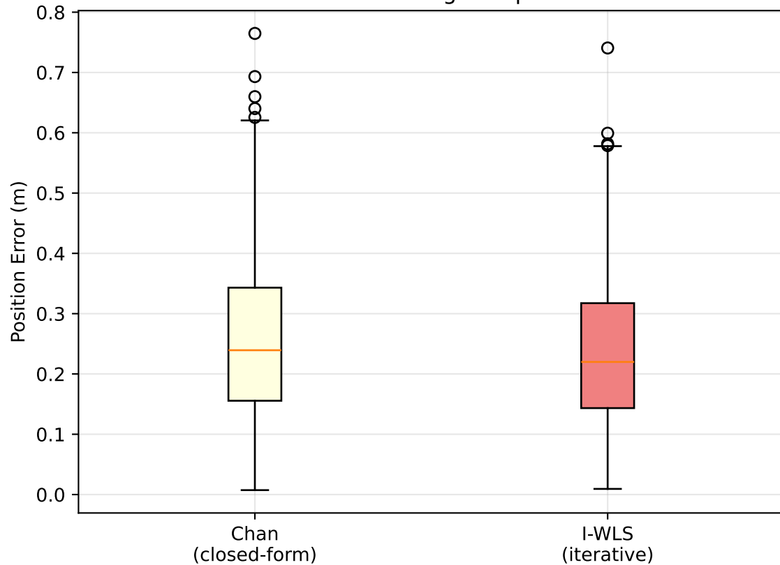
TDOA Positioning Comparison
