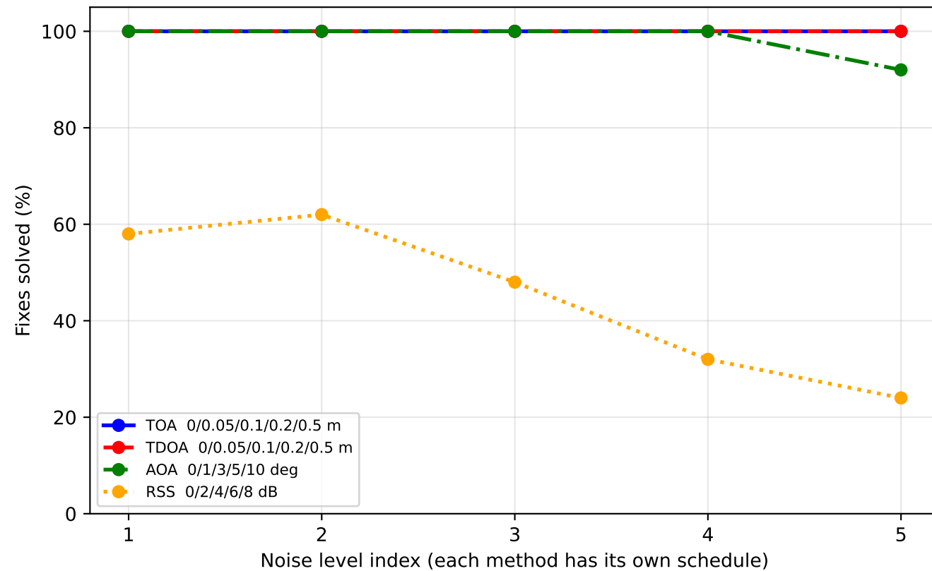
Fixes solved vs noise level (raised, refused, stalled at the seed, or >100 m all count as failed)
