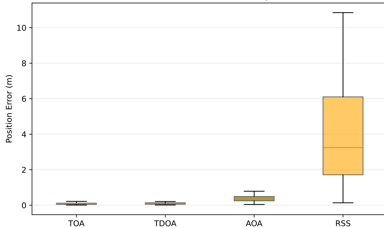
Error distribution at level 3 (TOA 0.1 m, TDOA 0.1 m, AOA 3 deg, RSS 4 dB)
