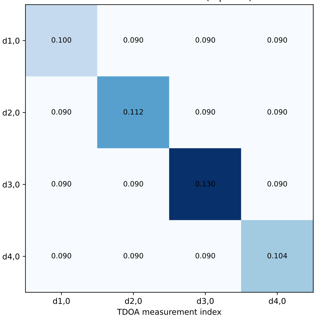
TDOA Covariance Matrix (Eq. 4.42)
