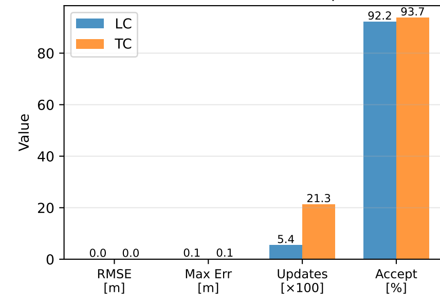
Performance Metrics Comparison
