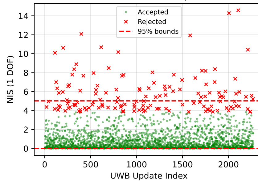
TC NIS (93.7% accepted)
