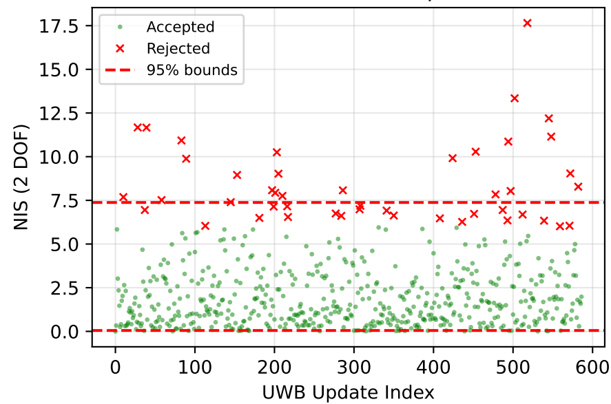
LC NIS (92.2% accepted)
