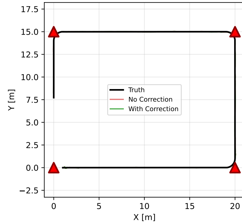
Direct Comparison
