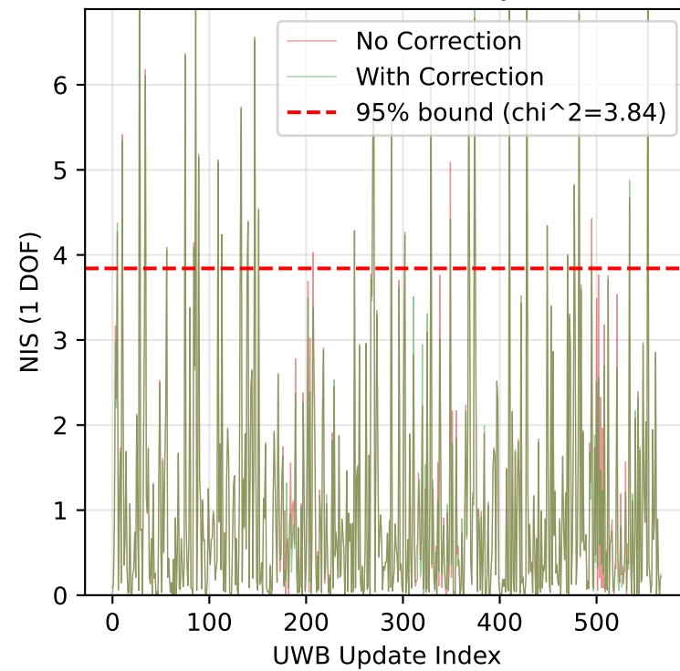
Innovation Consistency (NIS)
