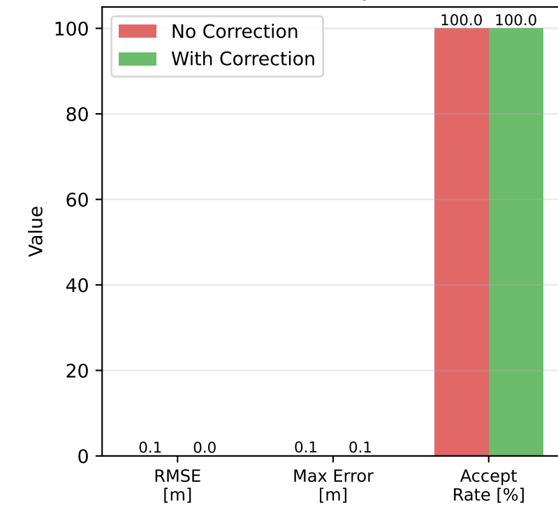
Metrics Comparison
