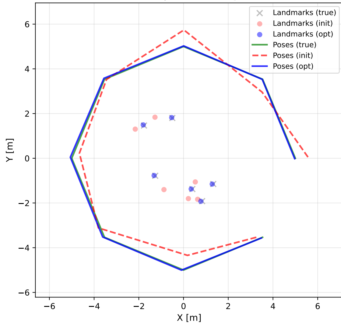
Bundle Adjustment: Top View
