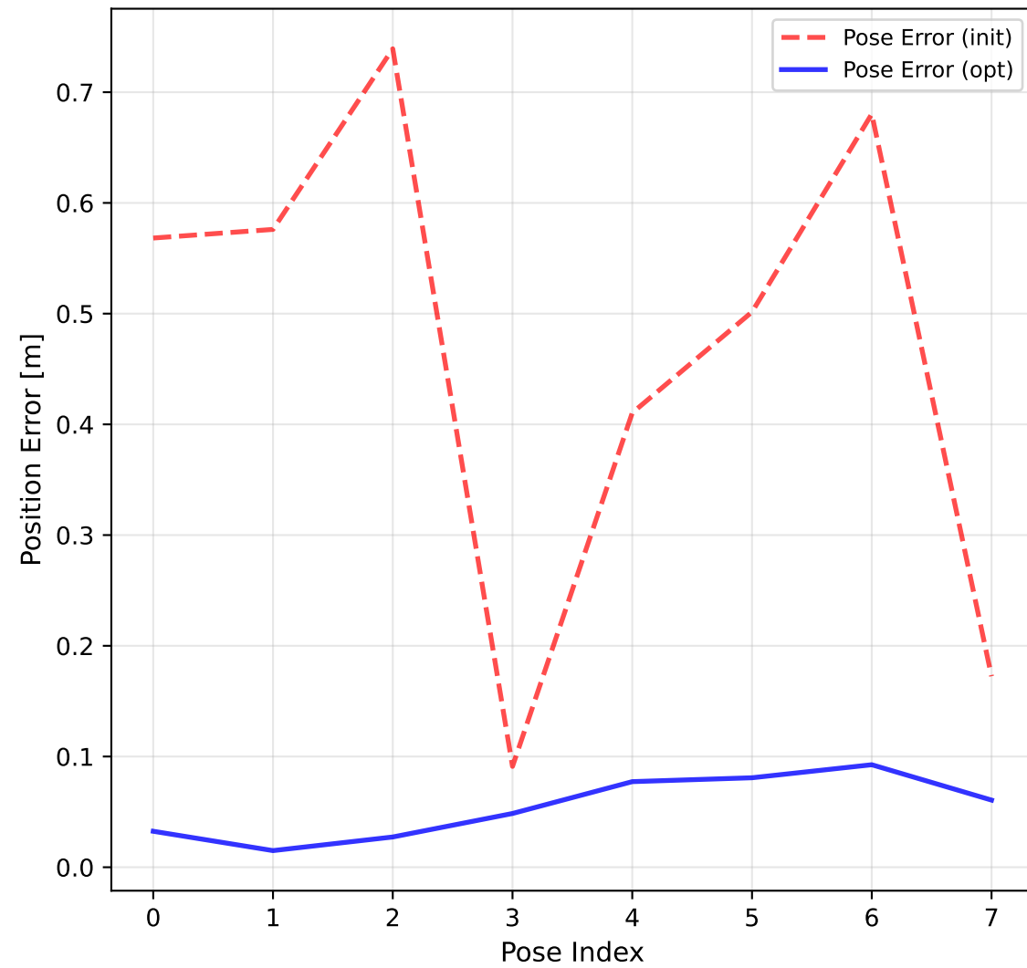
Camera Pose Errors
