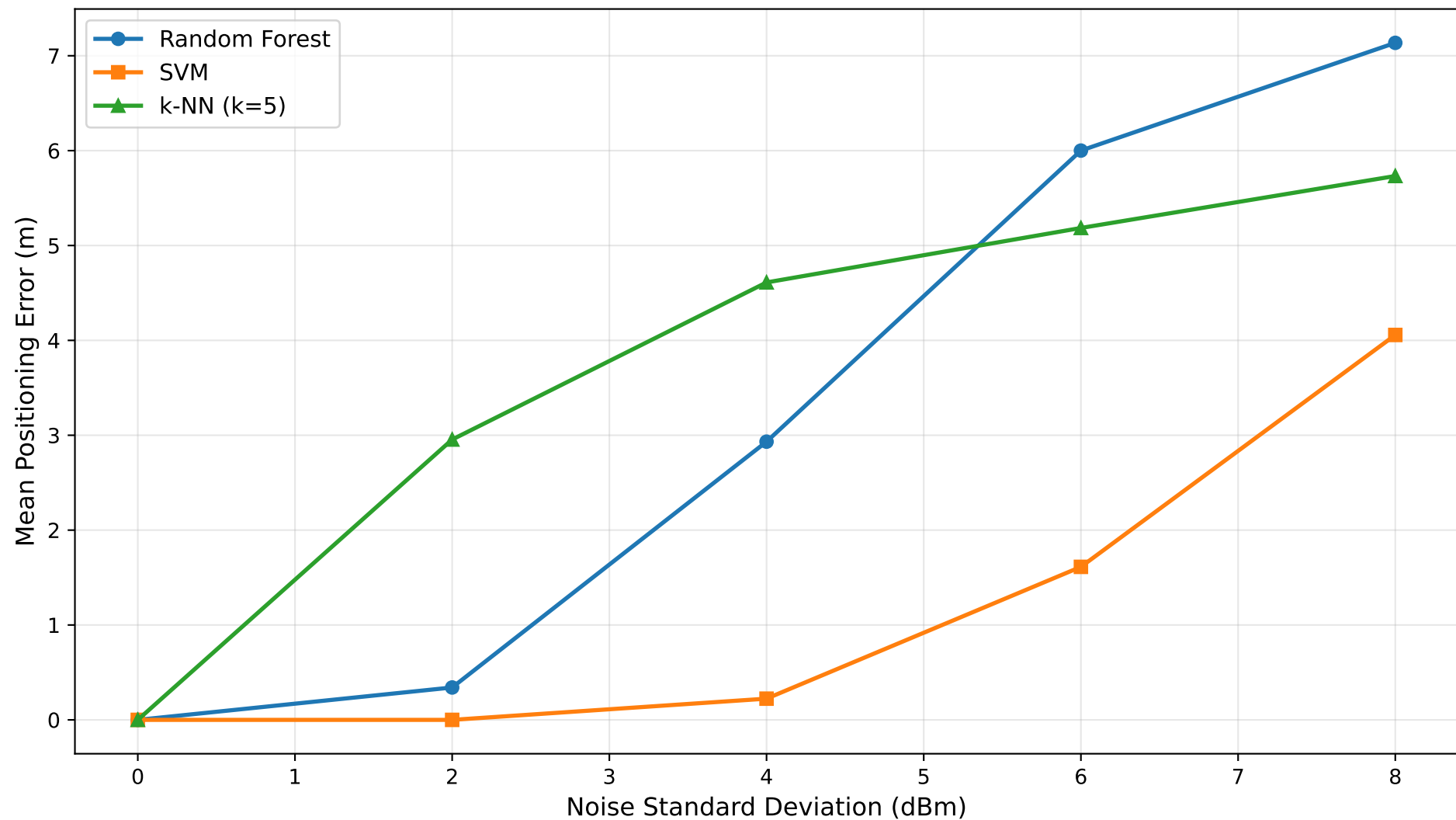
Classification vs k-NN: Robustness to Noise
