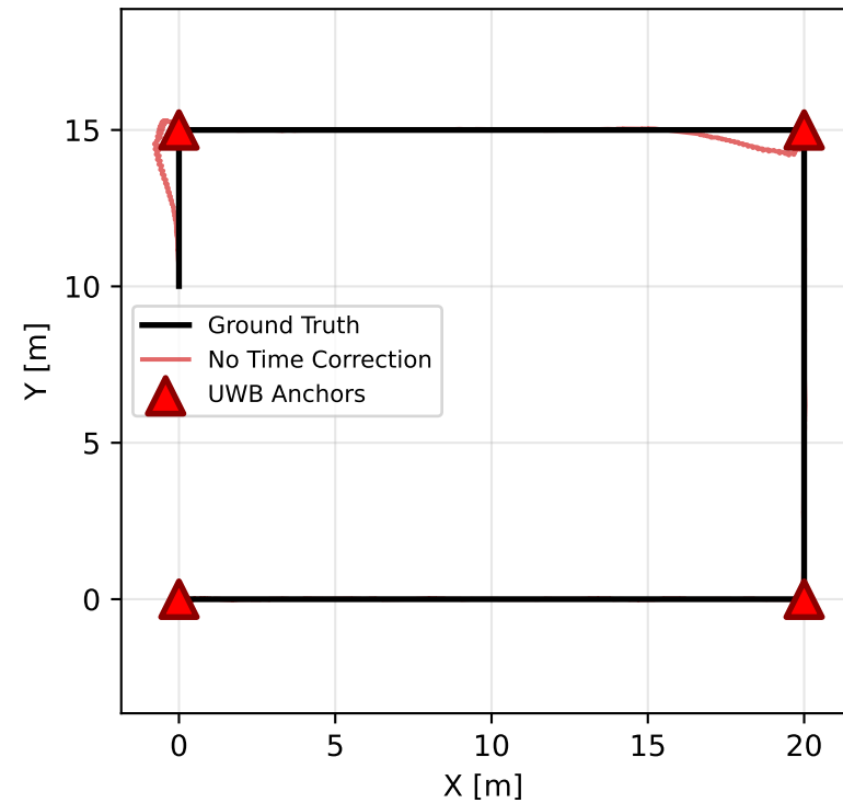
Without Correction (offset=-50ms, drift=100ppm)
