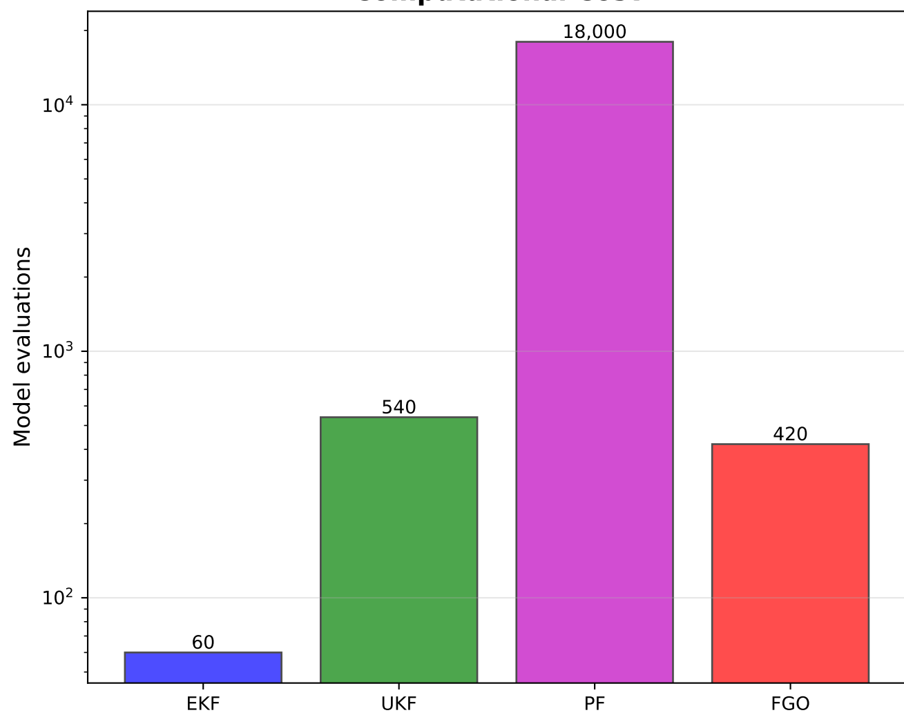
Computational Cost
