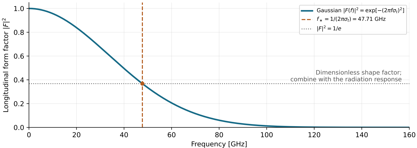
Case 1: full-bunch-length response, \sigma_z = 1 mm
