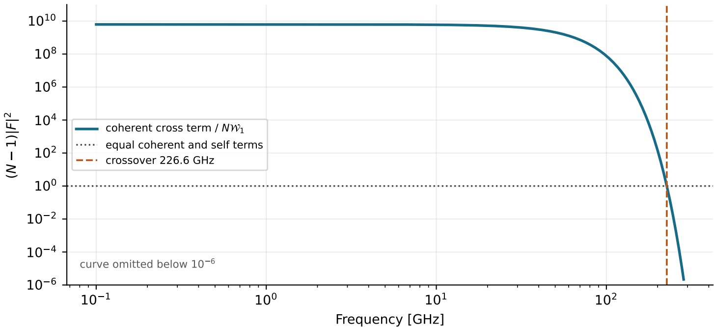
Gaussian bunch statistics for 1 nC and \sigma_z = 1 mm
