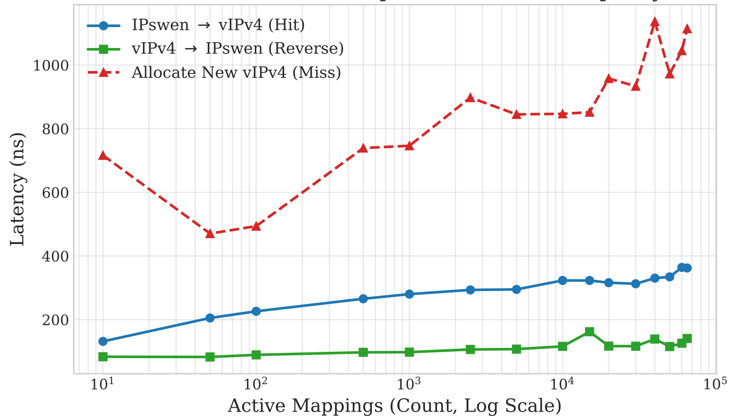
Address Translation Map Performance vs Capacity
