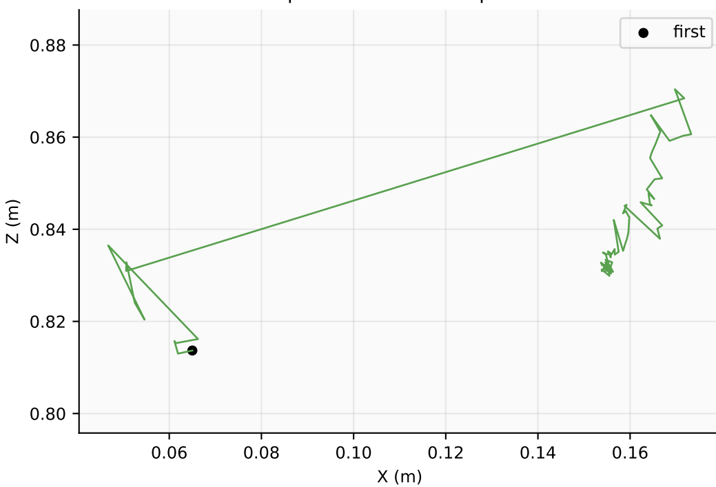
Composed world-board position
