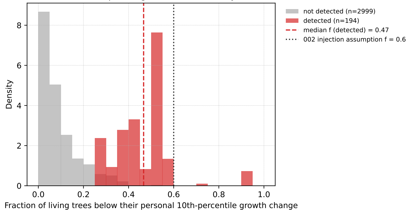
Tree-level responding fraction at event years
