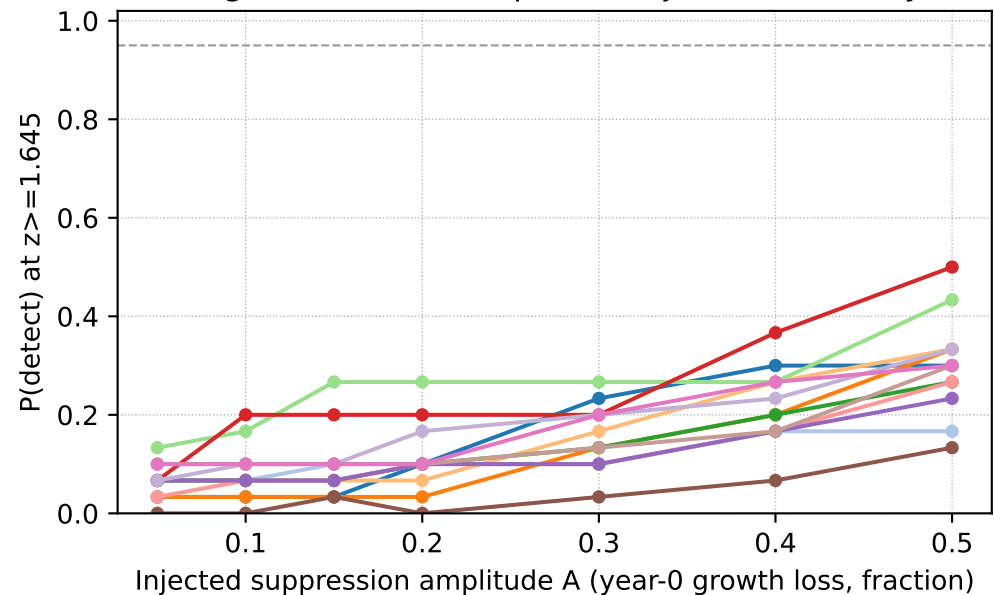
Single-site detection power (injection-recovery)
