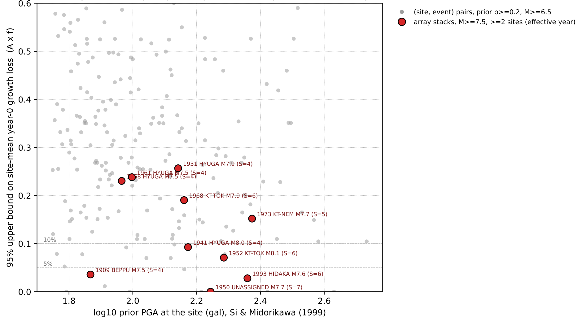
Far-field tree-ring insensitivity to great Japanese earthquakes (ITRDB array, 13 sites)
