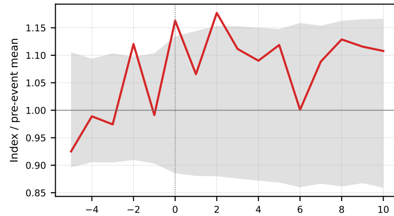
Teshio (n=4, p=0.173)
