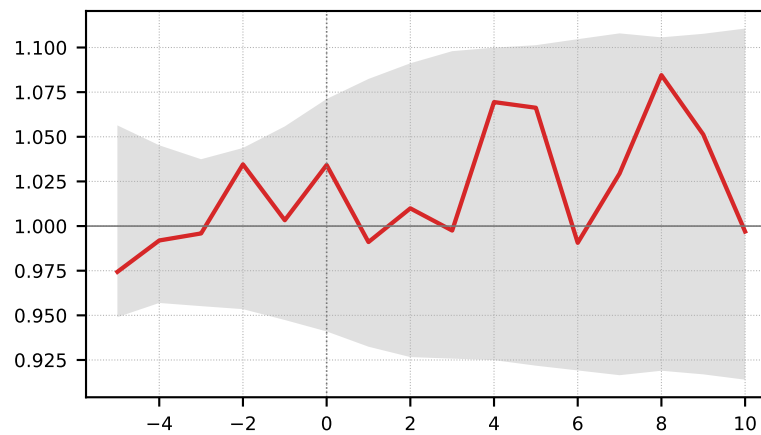
Yakushima A (n=3, p=0.413)
