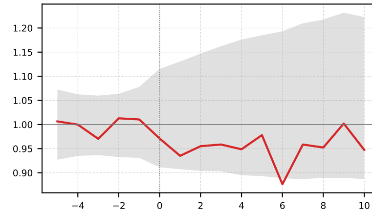
Tokachi (n=13, p=0.572)
