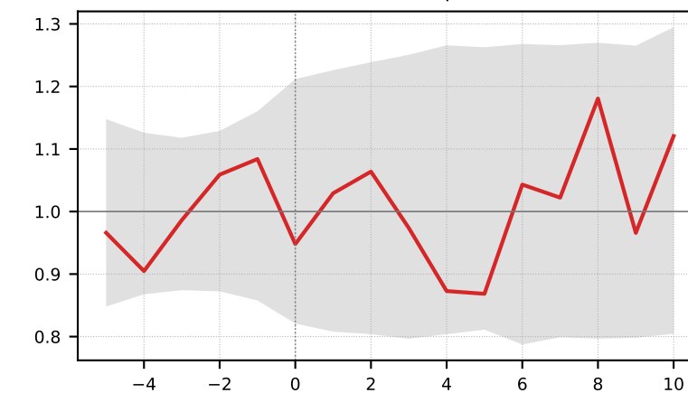
Yakushima (merged) (n=2, p=0.434)
