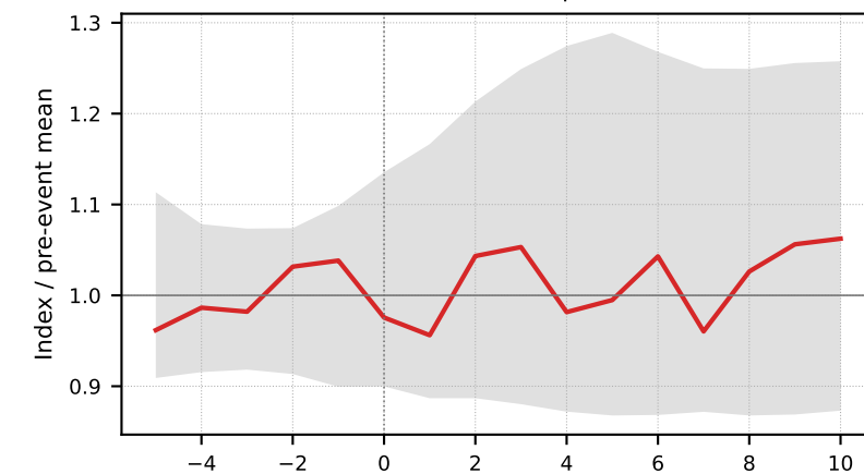
Yakushima C (n=2, p=0.322)
